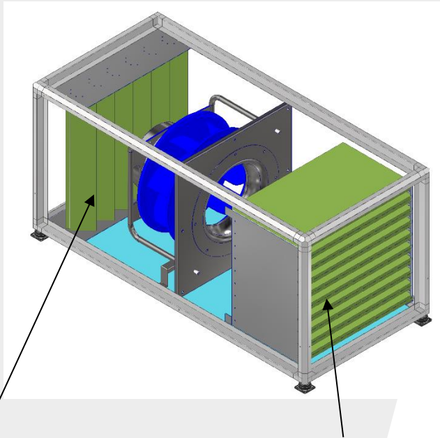
SOUND ABSORBING PANELS IN SUCTION
